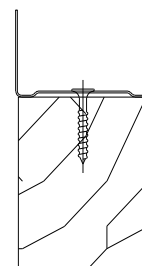
4- Rail R48 + traverse bois 58x46mm
