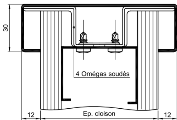
CLOISON A OSSATURE METALLIQUE
