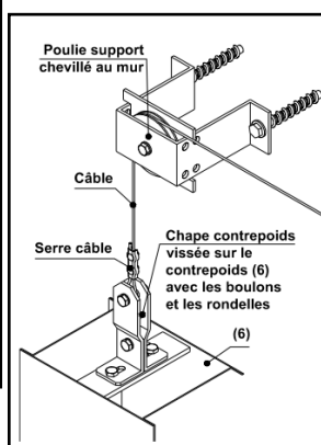
Kit poulie tirage direct
