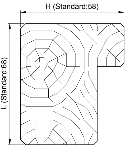
Section standard
