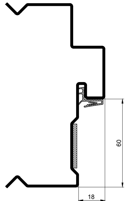
Joint K5499
