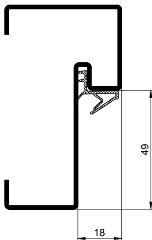
Joint K5499
