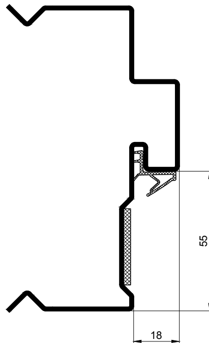
Joint K5499
