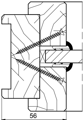
Double parclosage
