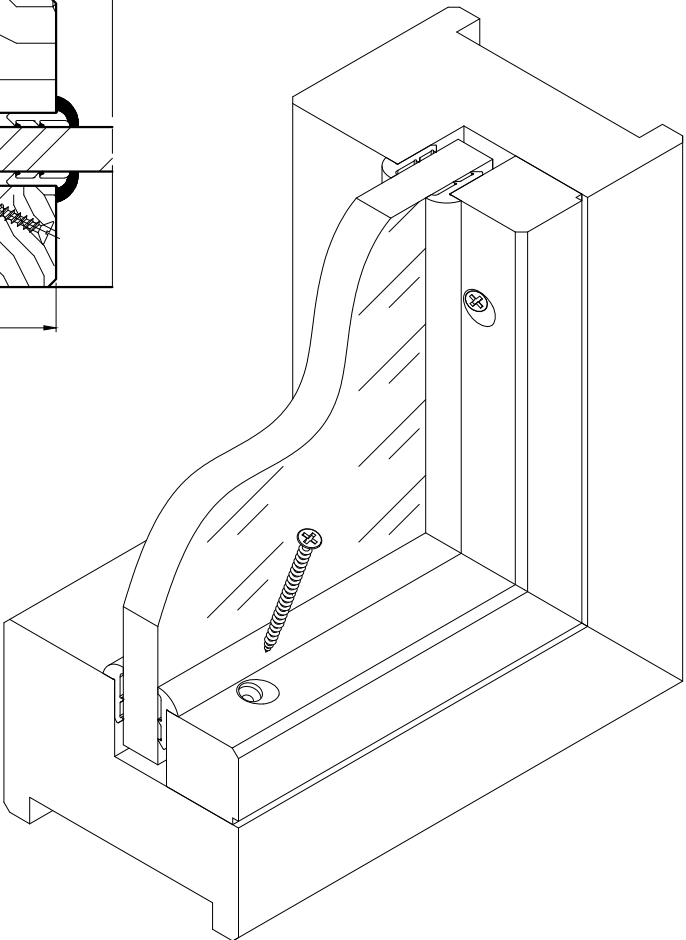
Double parclosage
