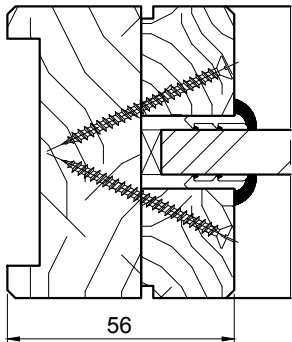
Double parclosage
