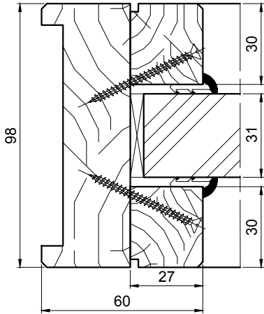
Double parclosage
