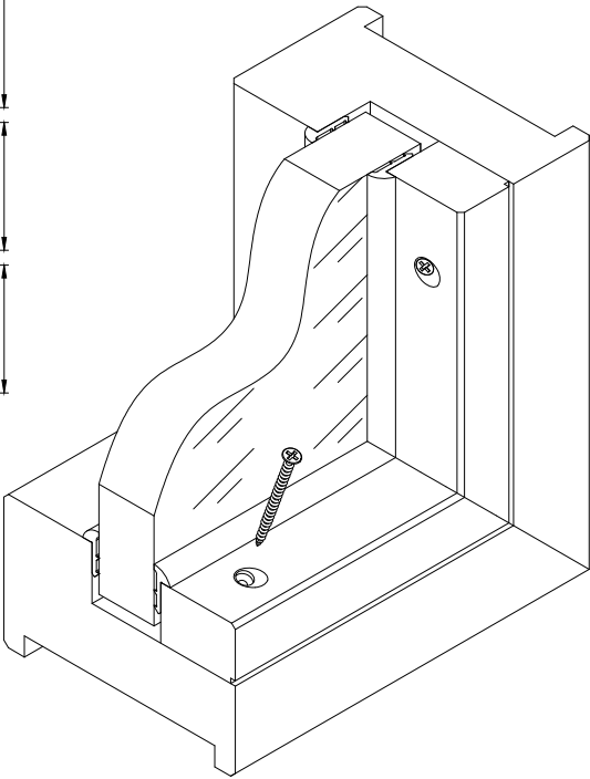
Parclosage standard
